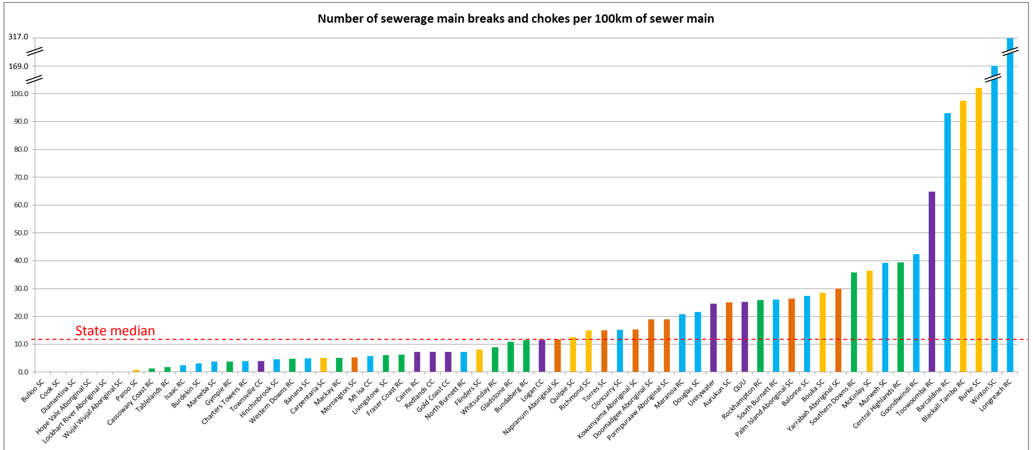
Figure 8. Number of sewerage main breaks and chokes per 100 km of sewer main 10 .
