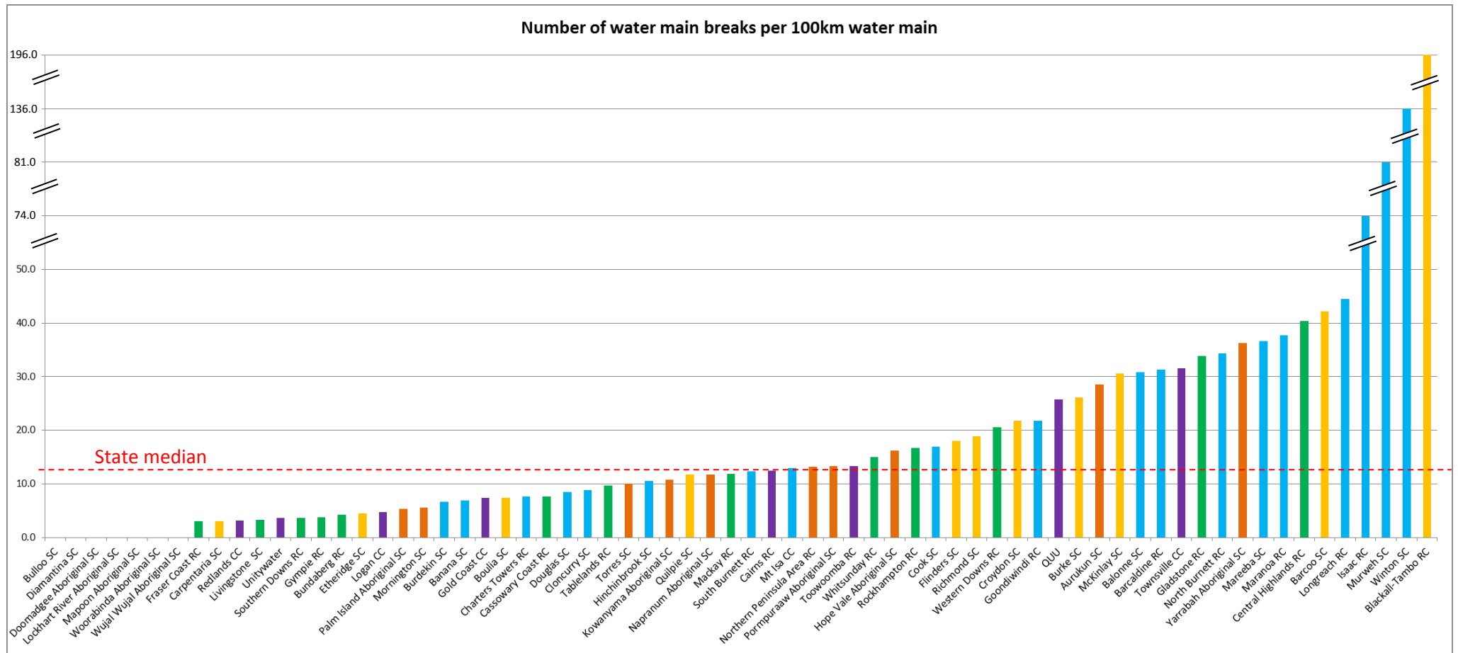
74 Figure 15. Number of water main breaks per 100 km of water main 18 .
