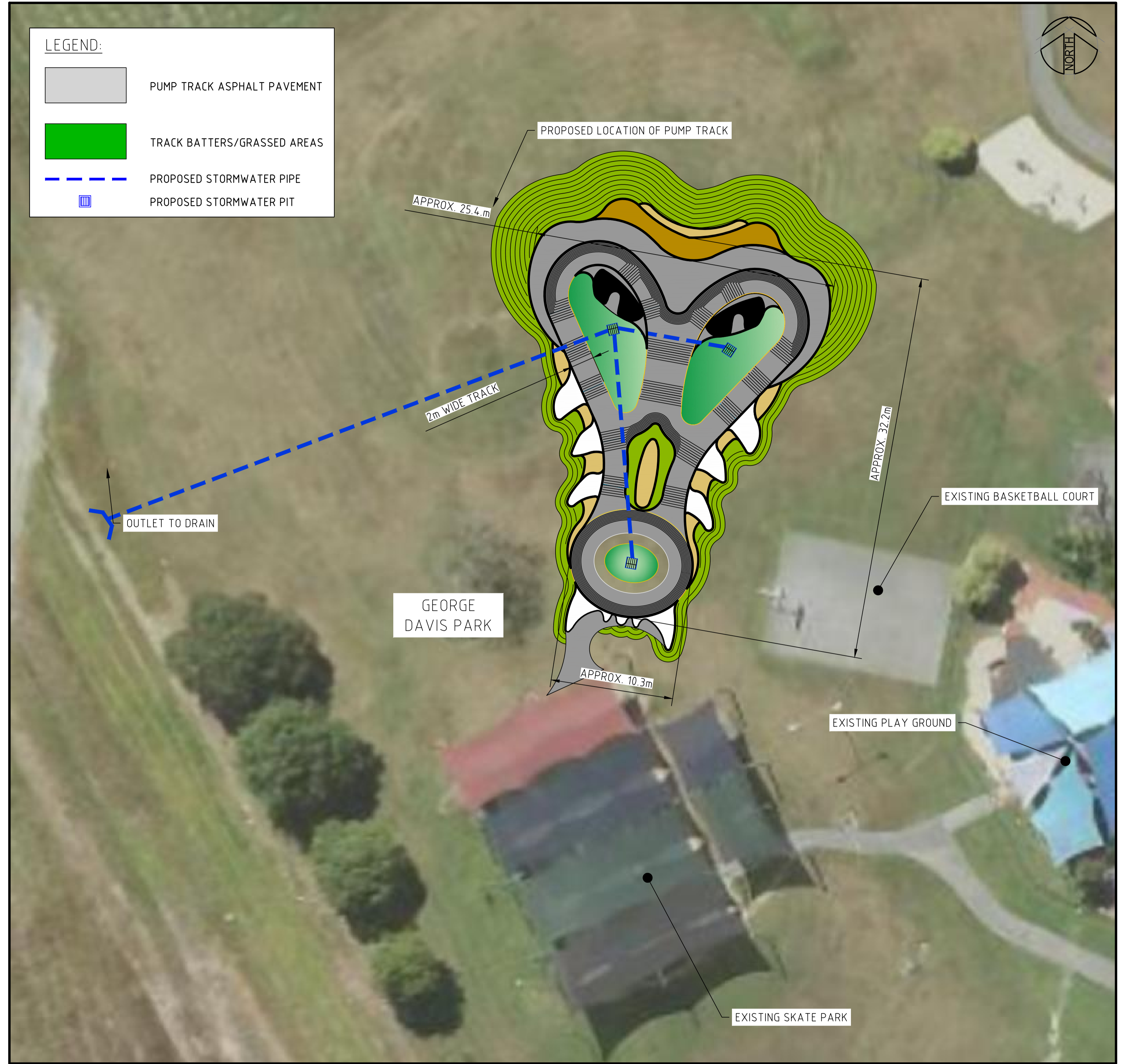
GENERAL ARRANGEMENT SCALE 1:200
