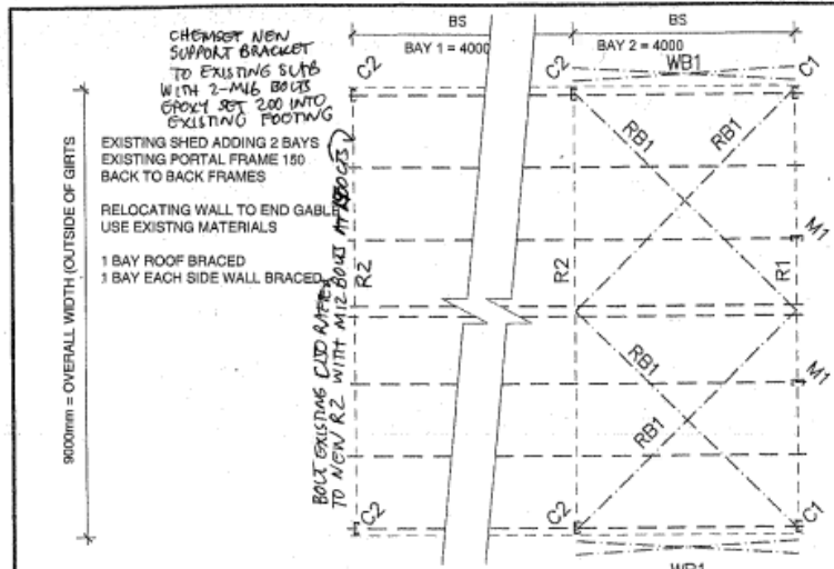
FRAMING PLAN NOT TO SCALE.
