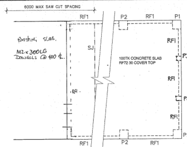
FOOTING PLAN NOT TO SCALE
