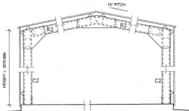
ELEVATION INTERNAL FRAME NOT TO SCALE
