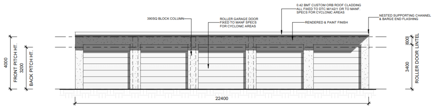
1 S04 FRONT ELEVATION 1 : 100
