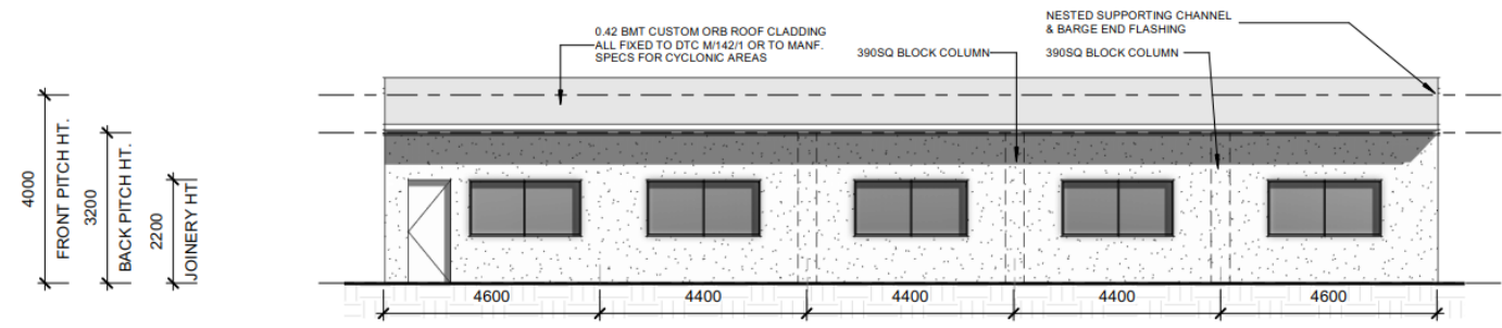
2 S04 REAR ELEVATION 1 : 100
