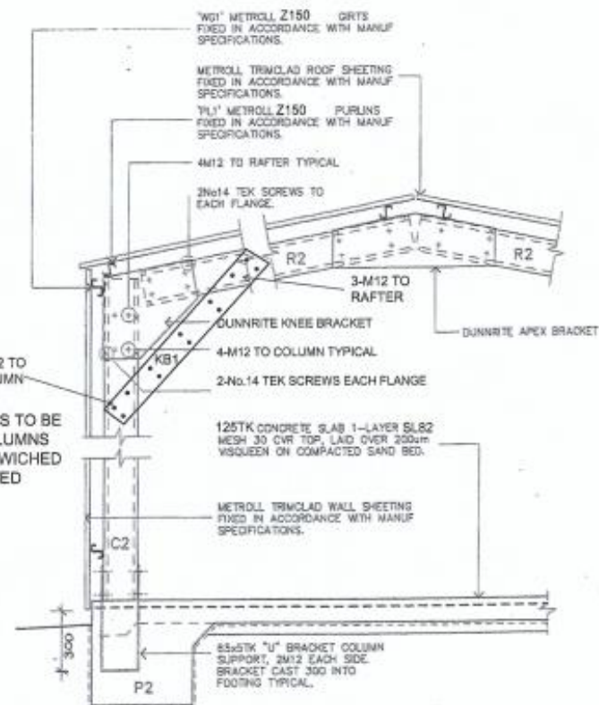
SECTION NOT TO SCALE
