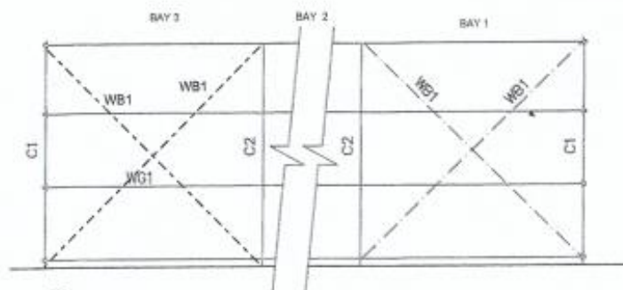
SIDE ELEVATION NOT TO SCALE
