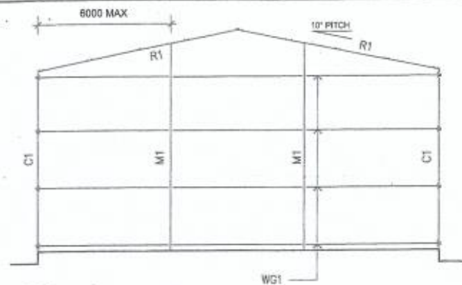
END ELEVATION NOT TO SCALE
