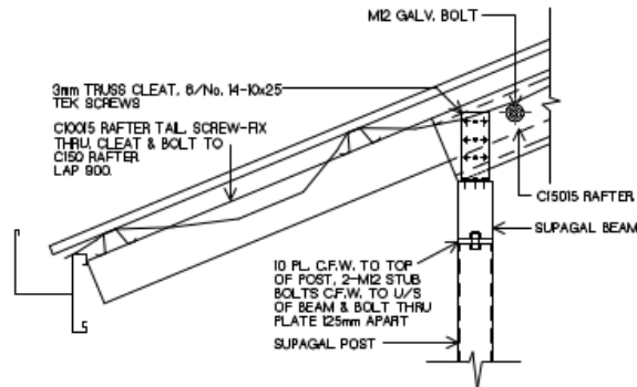
DETAIL TD1
