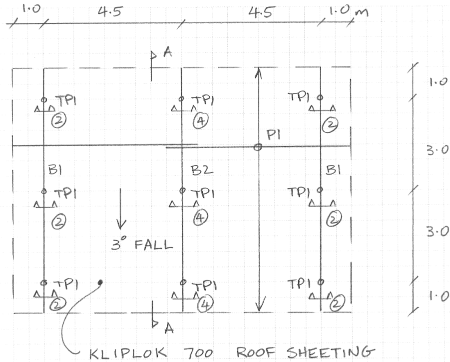
SHED ROOF PLAN (OPEN UNDER)
