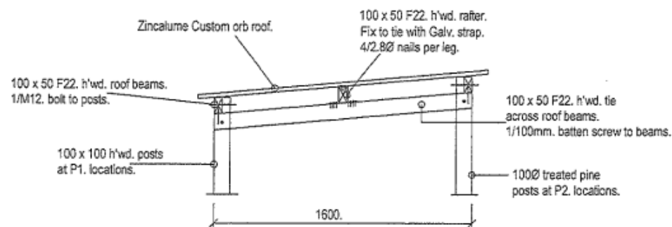
WALKWAY ROOF SECTION. 1:20.
