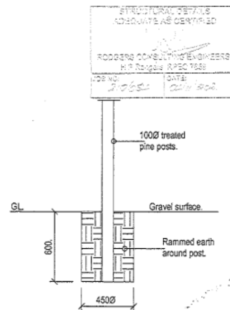
FOOTING P2. 1:20.
