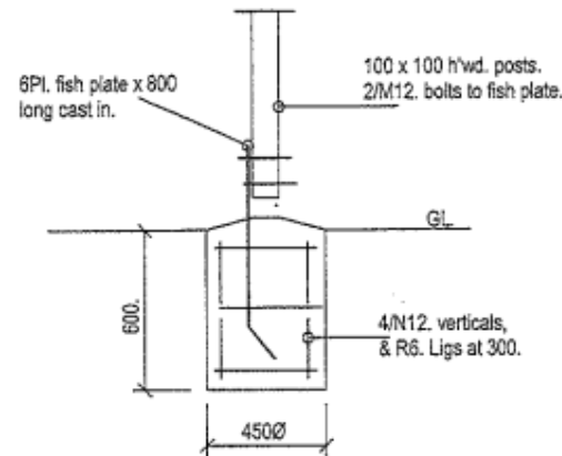
FOOTING P1. 1:20.
