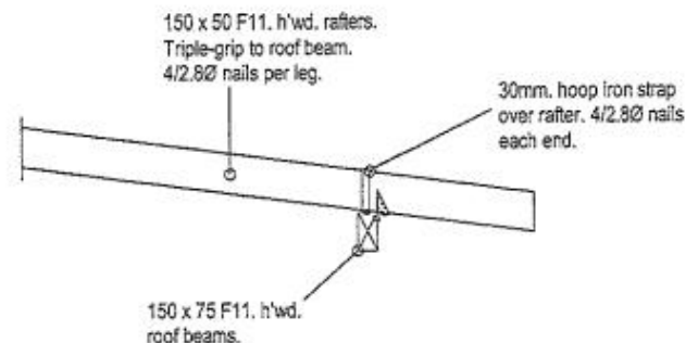
DETAIL B. 1:20.
