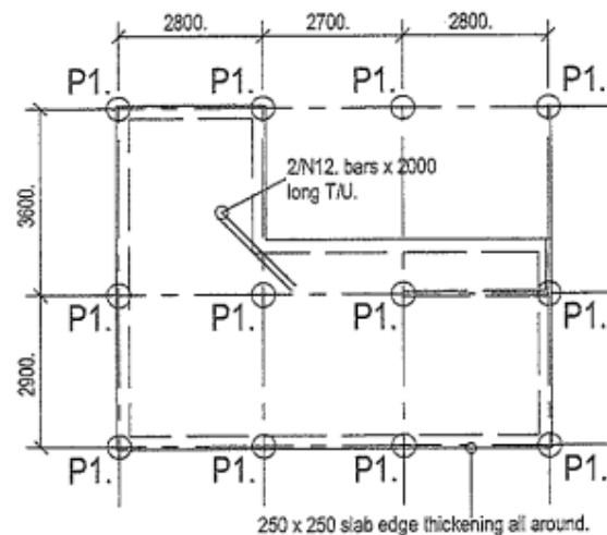
FOUNDATION PLAN.
