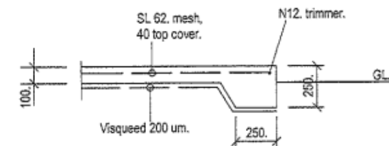
SLAB EDGE THICKENING 1:20.
