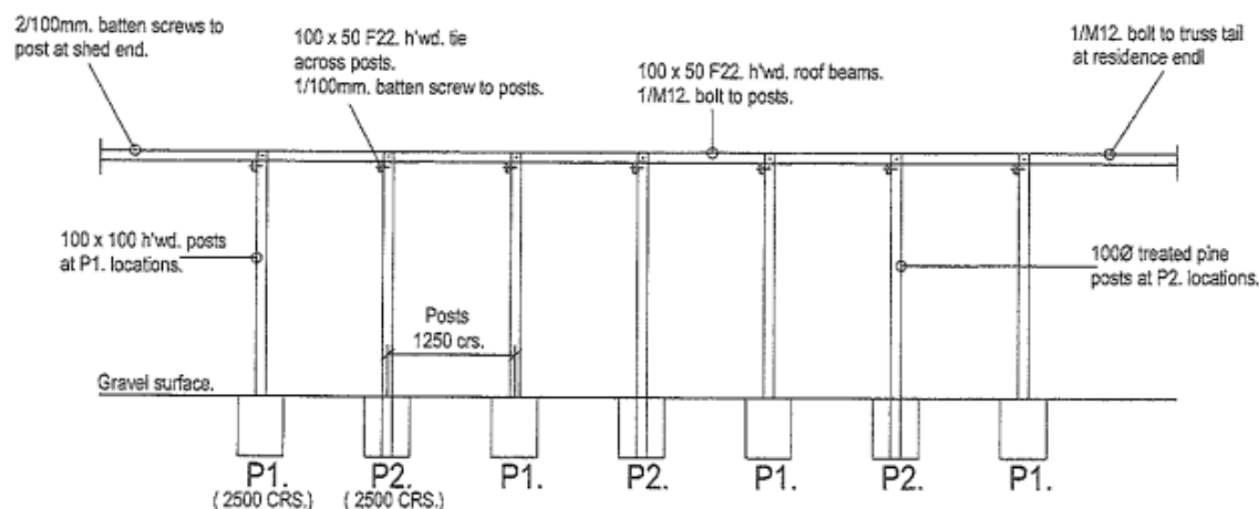
WALKWAY. 1:50.
