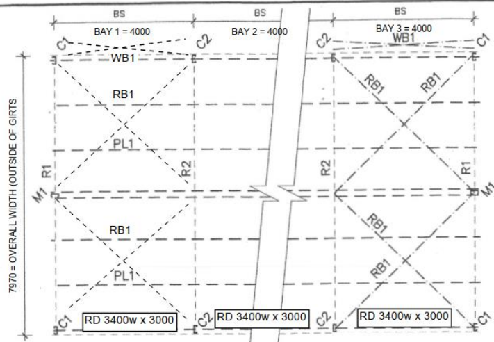
FRAMING PLAN NOT TO SCALE.
