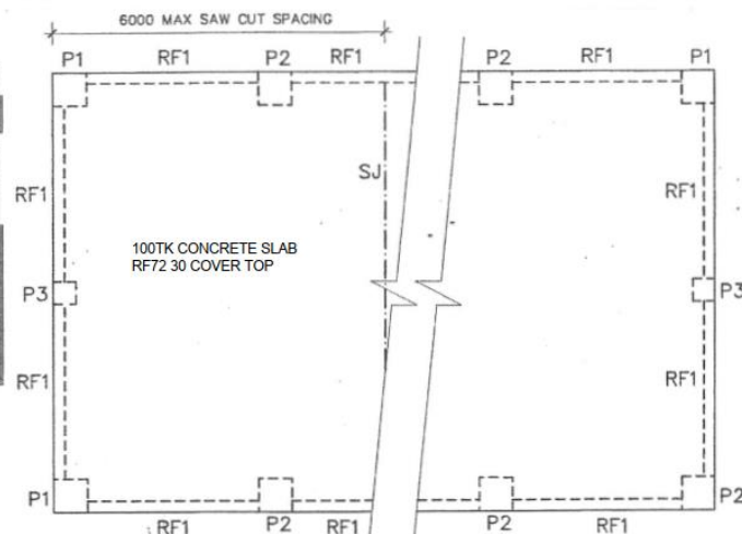
FOOTING PLAN NOT TO SCALE
