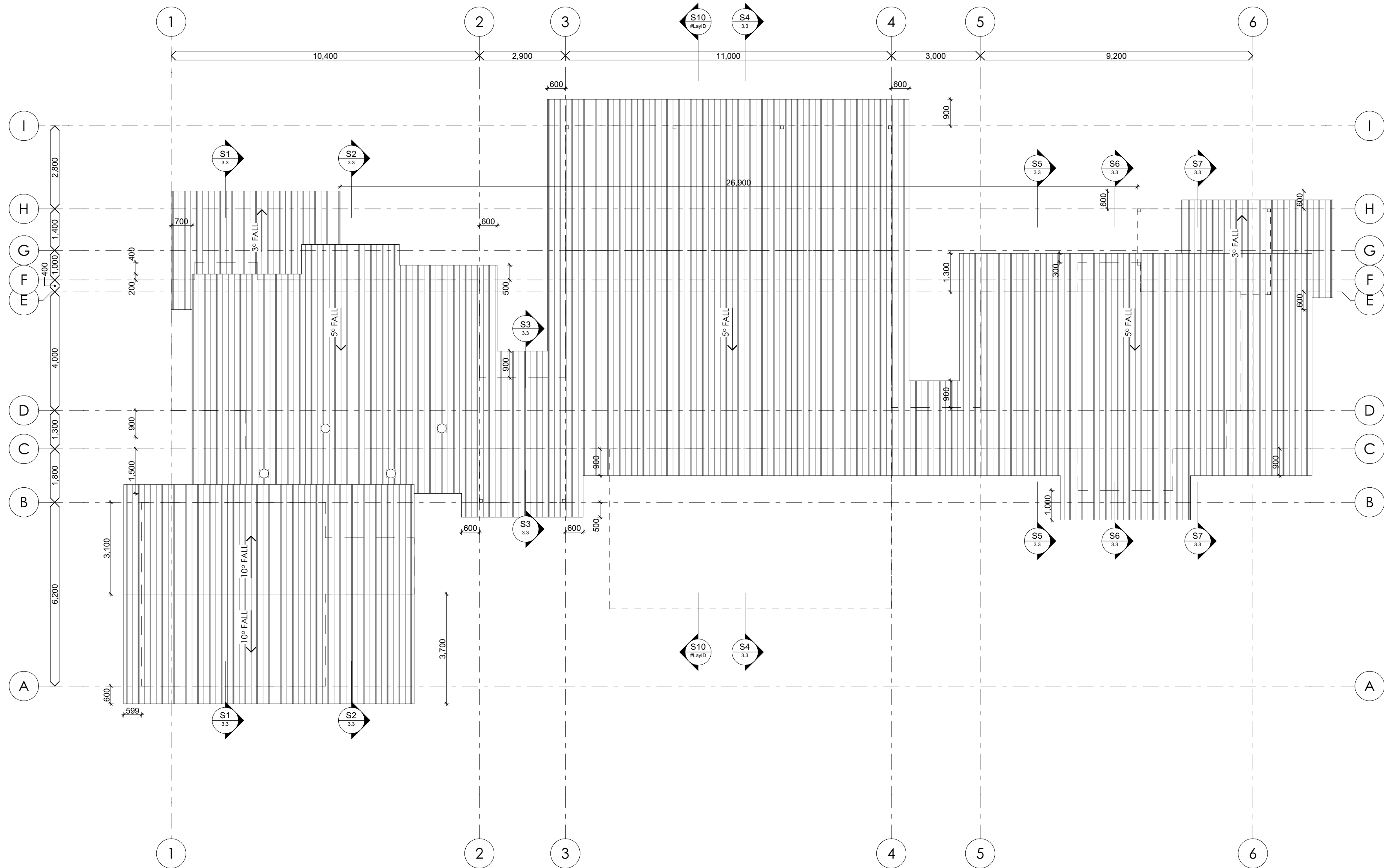
ROOF PLAN - PRIMARY RESIDENCE 1:100
