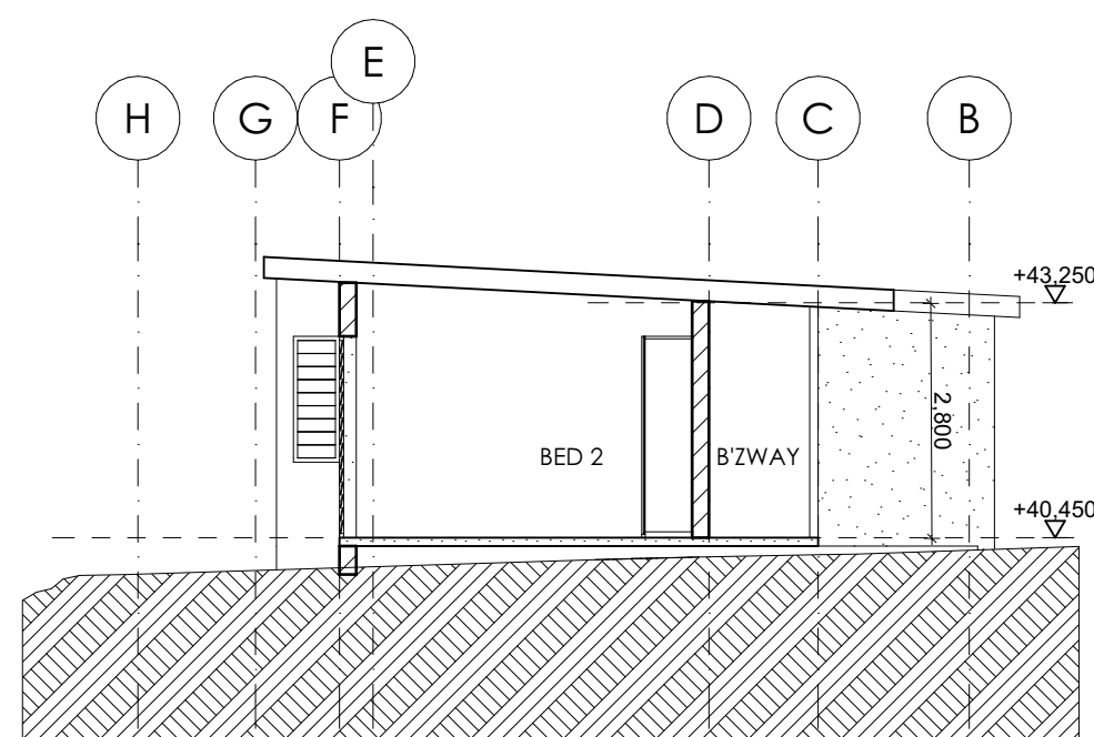
SECTION S5 1:100
