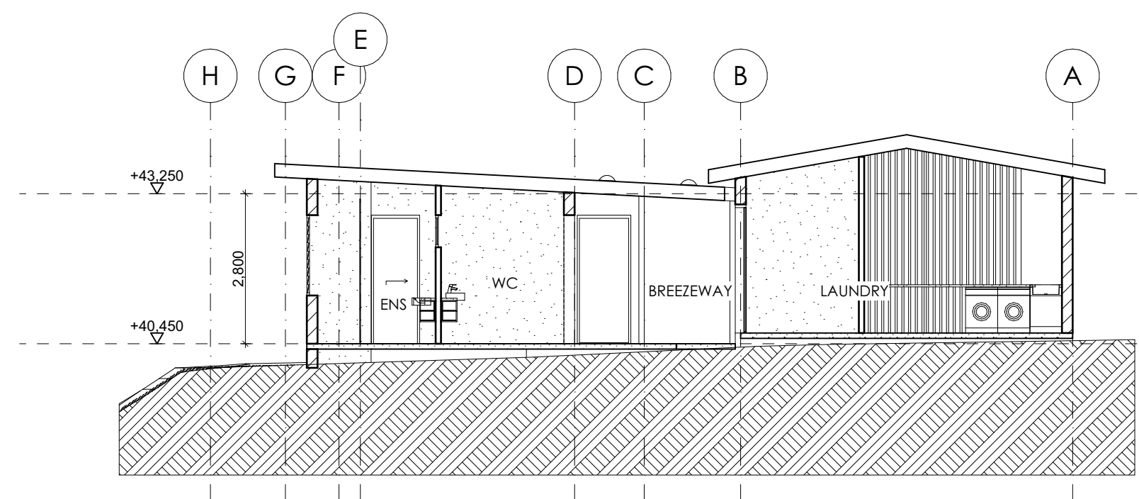
SECTION S2 1:100
