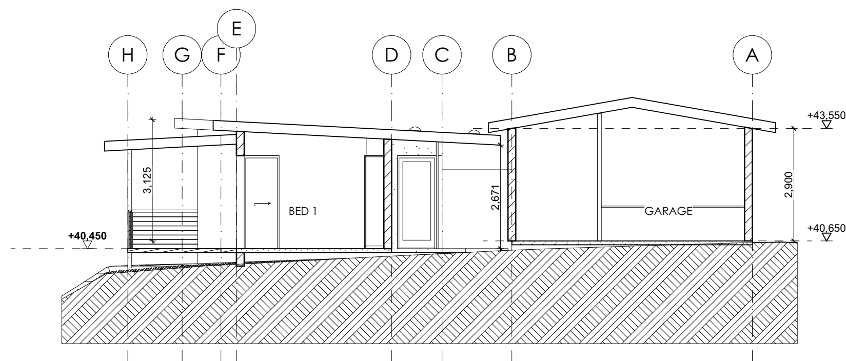
SECTION S1 1:100
