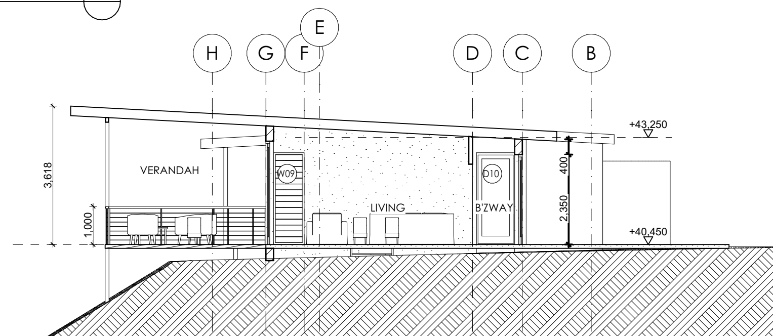
SECTION S4 1:100
