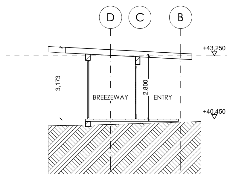
SECTION S3 1:100
