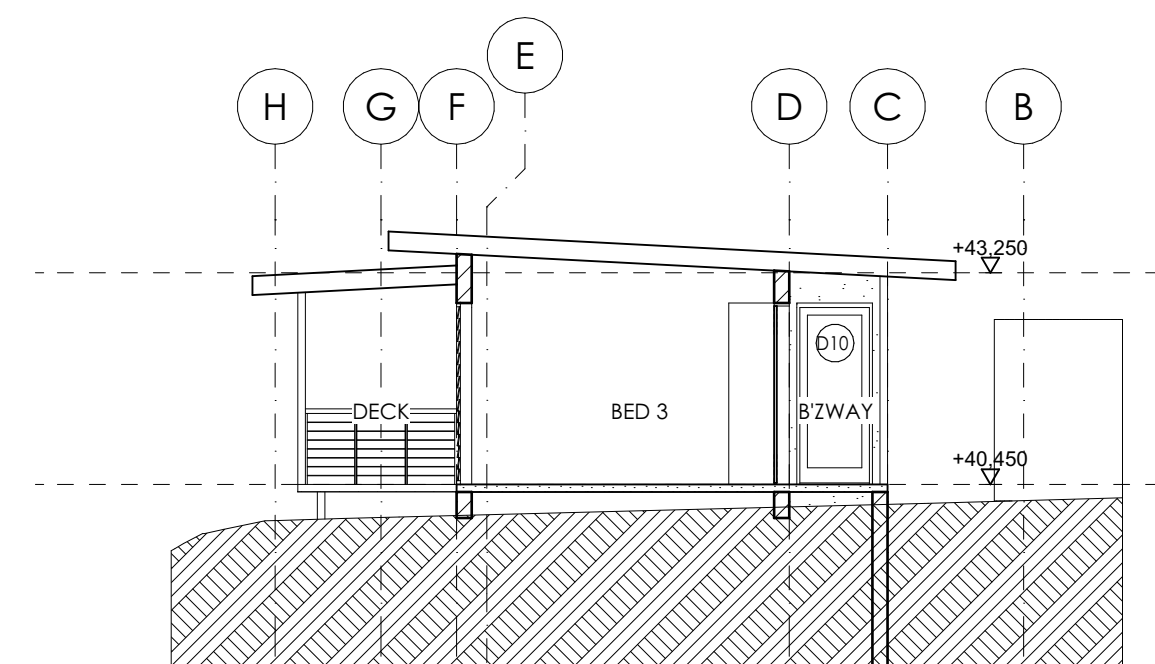
SECTION S7 1:100
