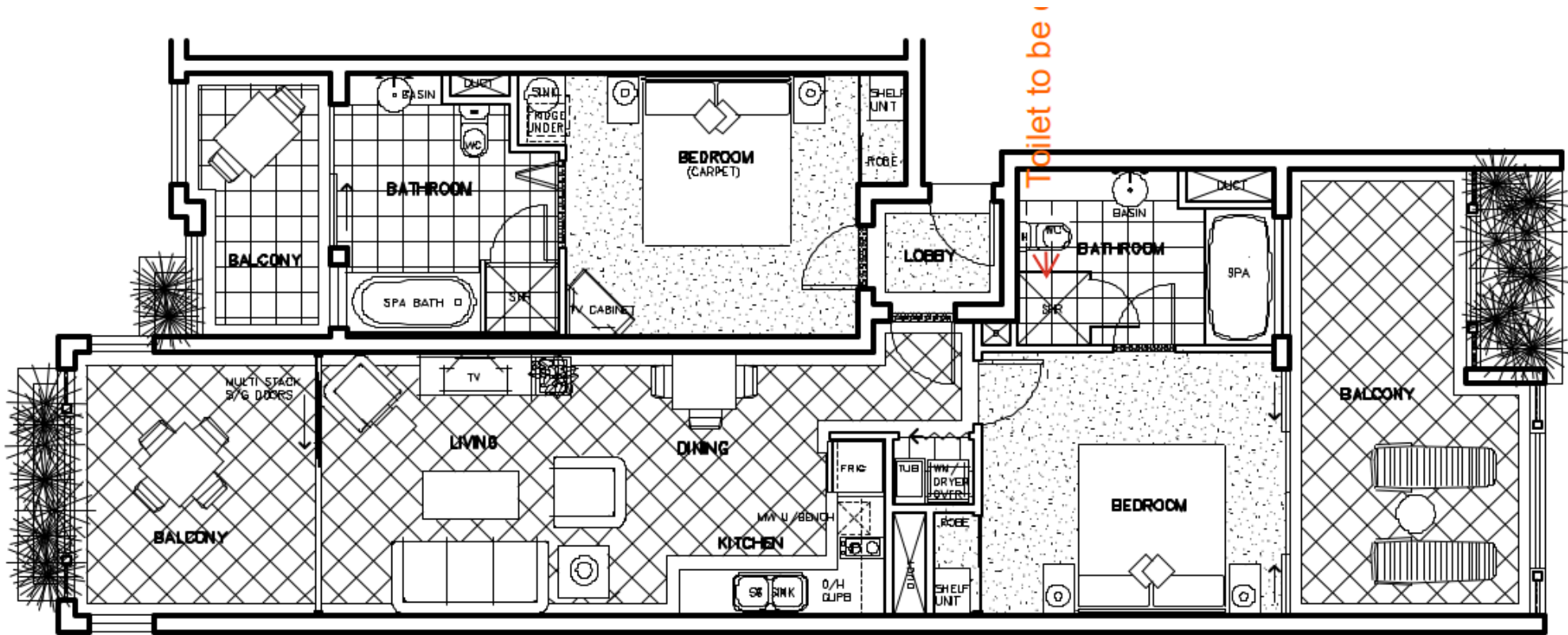
FLOOR PLAN TYPE E – "TWO-VIEW" DUAL OCCUPANCY APARTMENTS UNIT 10 MIRROR REV UNIT 11
