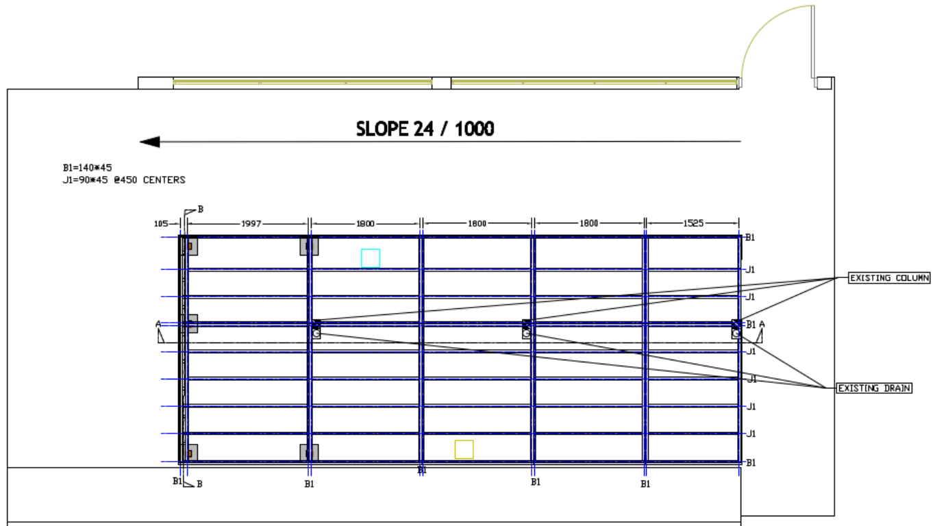
Sub-frame Floor Plan Scale 1:50
