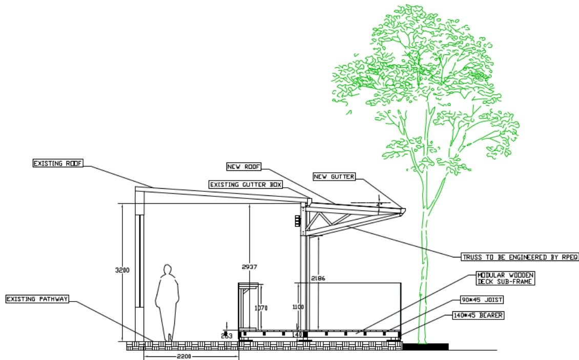
SECTION B-B Scale 1:50
