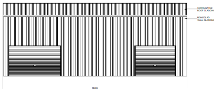
1 SIDEWALL EXTERIOR ELEVATION SCALE: 1 = 100
