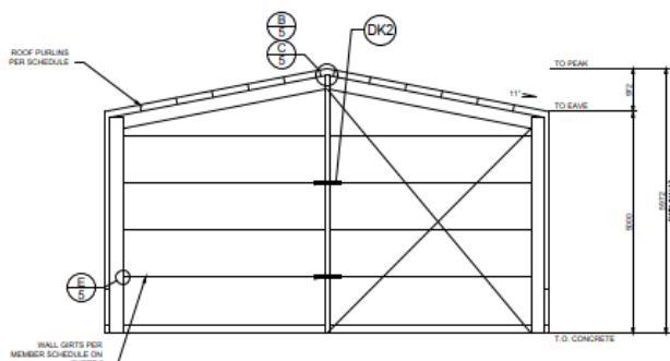
4 ENDWALL INTERIOR ELEVATION SCALE: 1/4"=1'-0"
