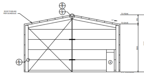
5 ENDWALL INTERIOR ELEVATION SCALE: 1/4"=1'-0"
