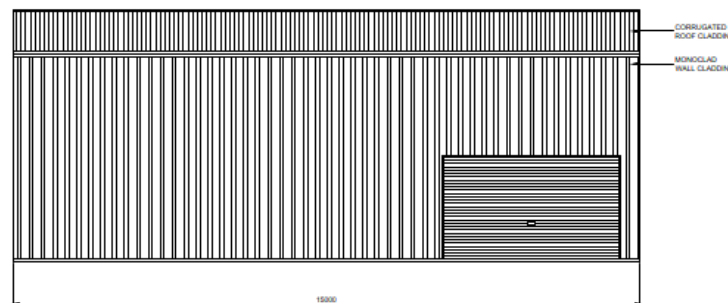
2 SIDEWALL EXTERIOR ELEVATION SCALE: 1 = 100
