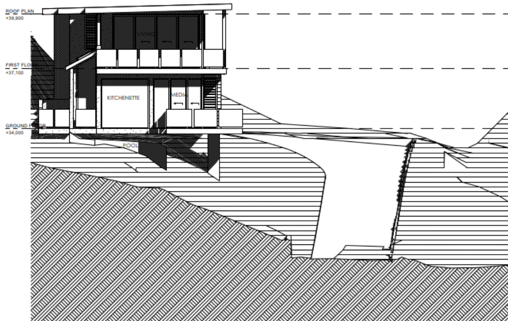
BOUNDARY ELEVATION 02 1:100
