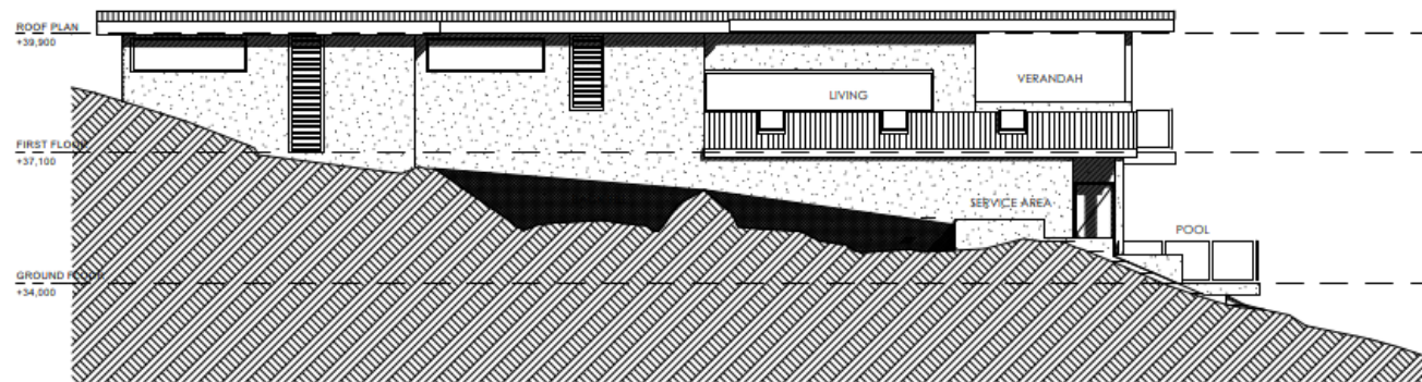
BOUNDARY ELEVATION 03 1:100
