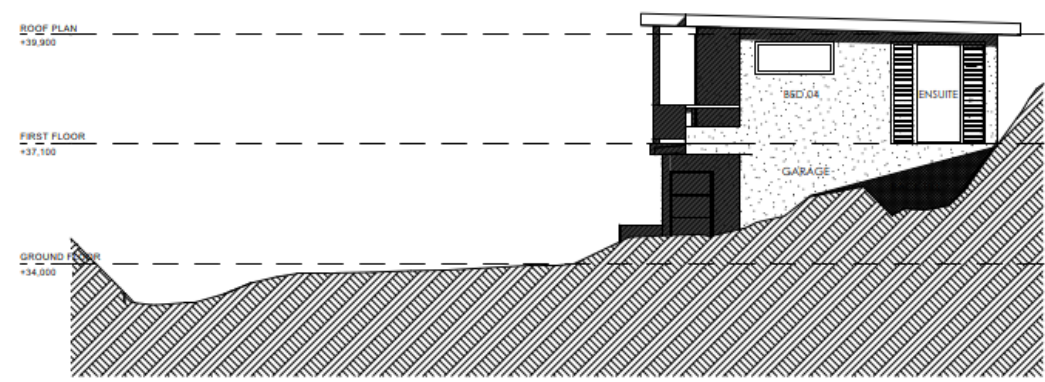
BOUNDARY ELEVATION 04 1:100
