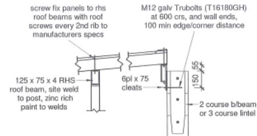
C Roof Panel Fixing 1 : 20
