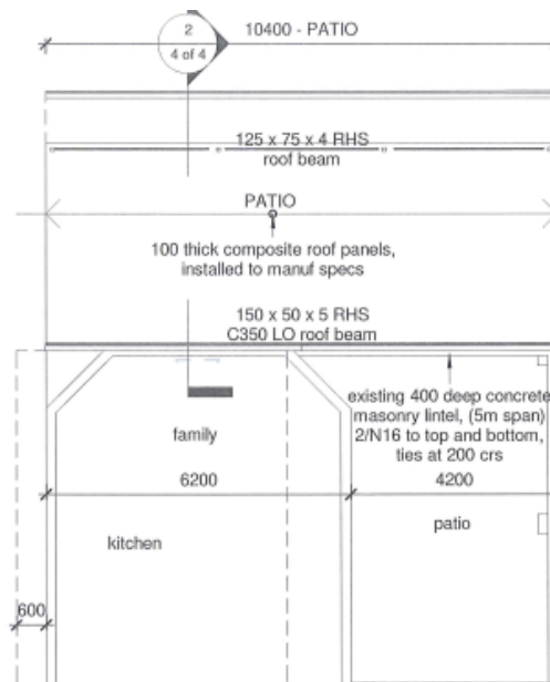
2 Roof Framing Plan 1 : 100
