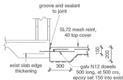
B T2 Footing 1 : 20
