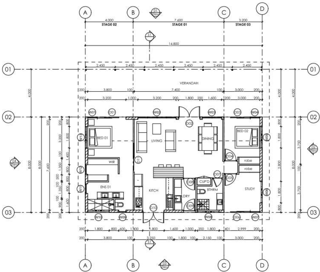
FLOOR PLAN 1:100
