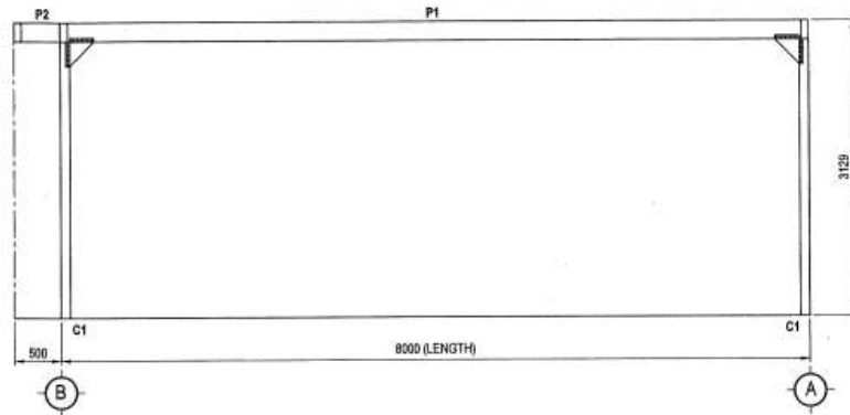
ELEVATION FRAMING GL.A SCALE 1:50
