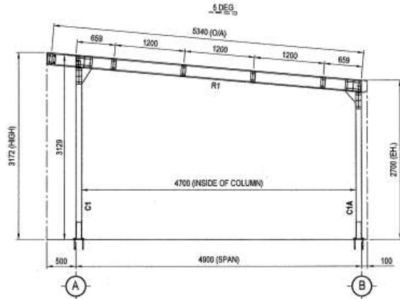
ELEVATION FRAMING GL.1 SCALE 1:50
