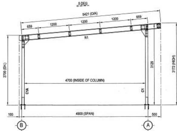
ELEVATION FRAMING GL.2 SCALE 1:50
