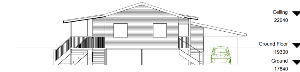
2 SOUTHWEST ELEVATION 1 : 100
