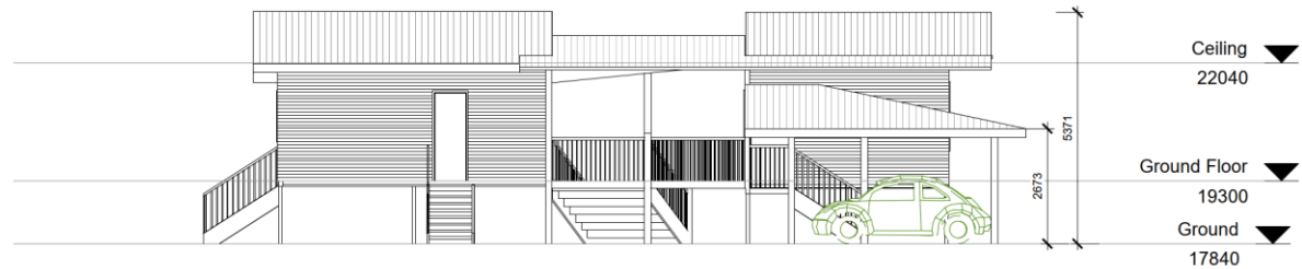
1 SOUTHEAST ELEVATION 1 : 100
