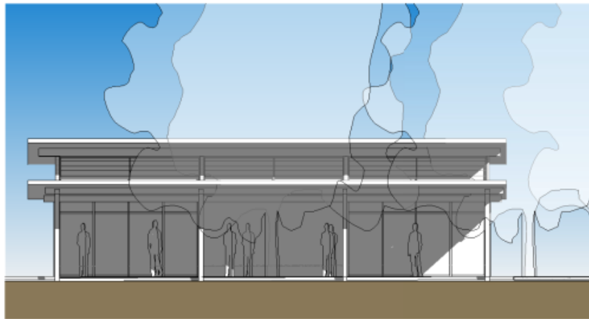
1 Front Elevation 1 : 100 @ A3
