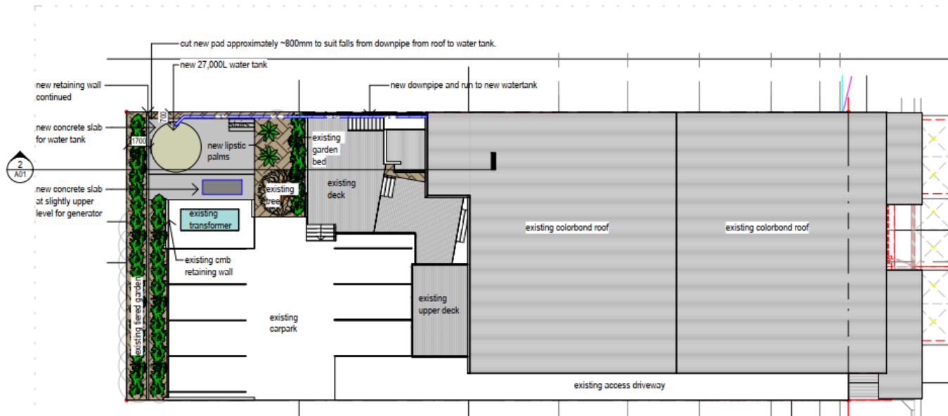
1 Site Plan 1: 200 @ A3
