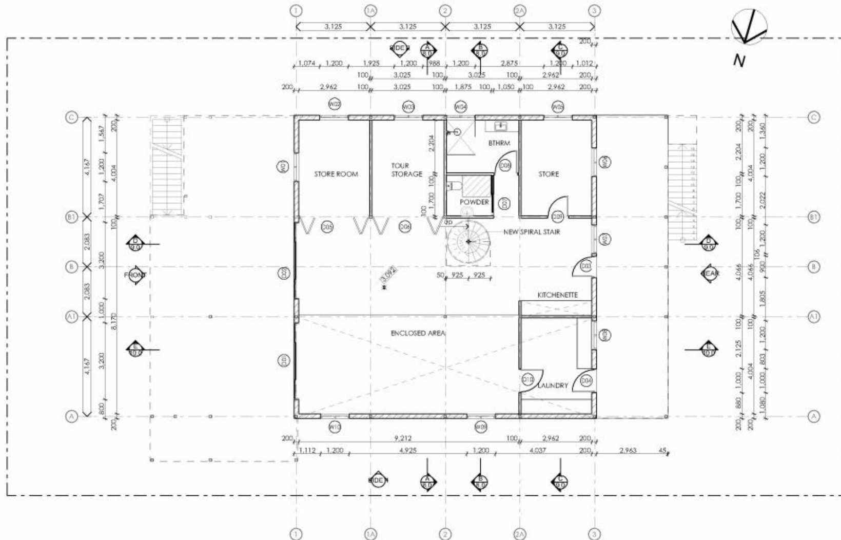
GROUND FLOOR 1:100
