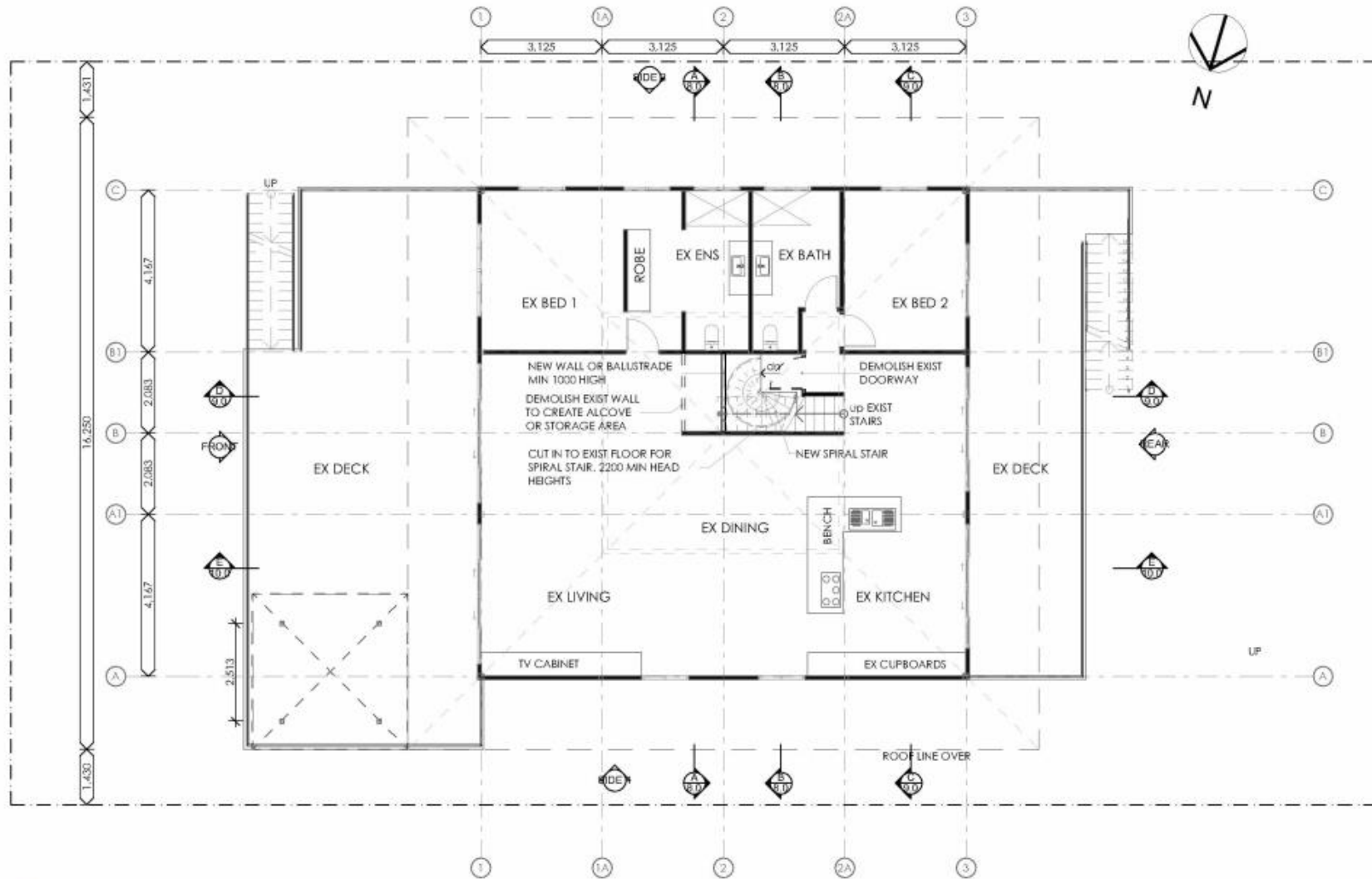
FIRST FLOOR 1:100
