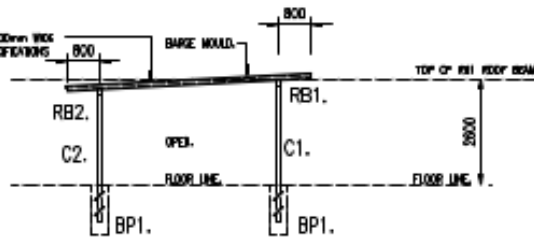
SOUTH-EAST ELEVATION. SCALE 1:100 NORTH-WEST ELEVATION SIMILAR.
