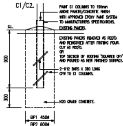
BP1 & BP2 DETAIL.
