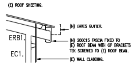
SECTION, SCALE :- 1:20 NEW EAVES GUTTER TO EXISTING SHED.
