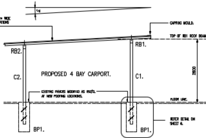
TYPICAL SECTION. SCALE 1:100
