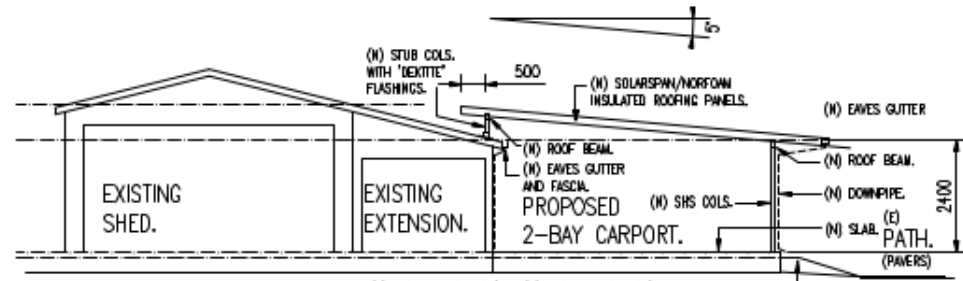
FRONT ELEVATION.
