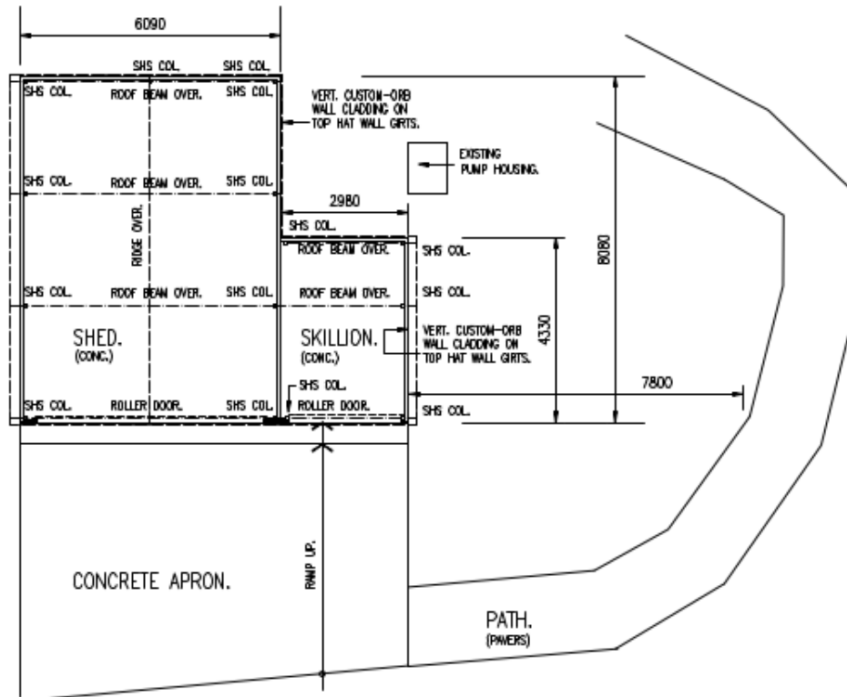
'EXISTING' SHED/SKILLION FLOOR PLAN.
