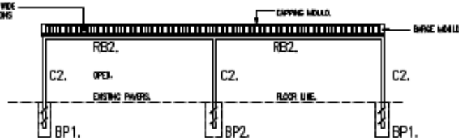
NORTH-EAST ELEVATION. SCALE 1:100 REAR ELEVATION. FROM HARTLEY'S DRIVE
