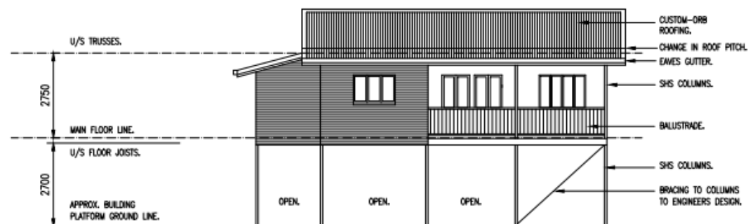
NORTH ELEVATION.
