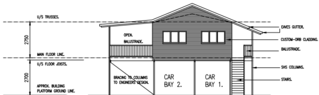
WEST ELEVATION.
