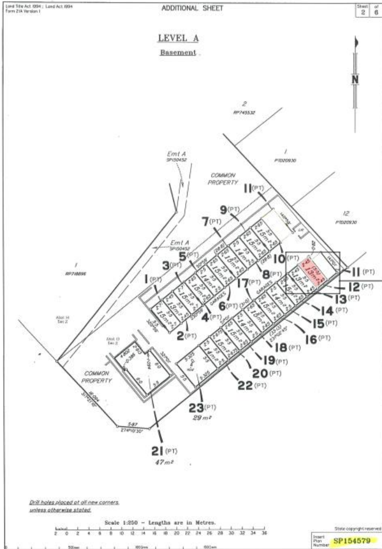
1 CARPARK LAYOUT
