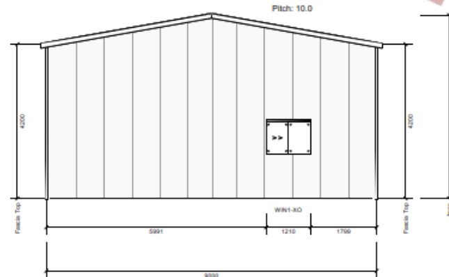
BACK ELEVATION
