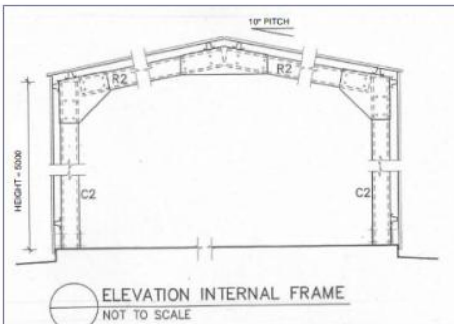
Figure 2: Shed Elevation (Extract from Approved Building Plans)
