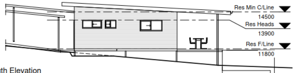
1 South Elevation 1 : 100
