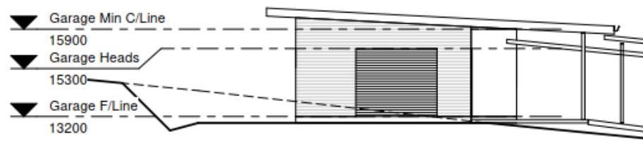
1 South Elevation 1 : 100
