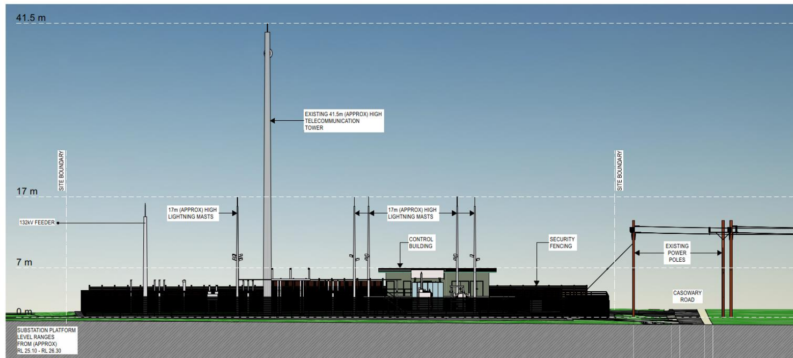
ELEVATION - NORTH 1:300
