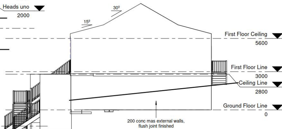
2 Right Elevation 1 : 100 (Left Elevation opposite)
