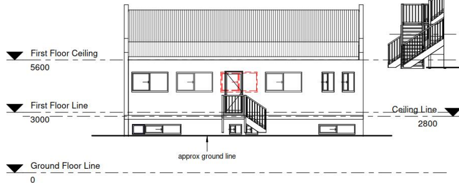
3 Rear Elevation 1 : 100
