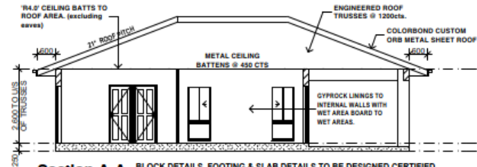
Section A-A BLOCK DETAILS, FOOTING & SLAB DETAILS TO BE DESIGNED, CERTIFIED AND INSPECTED BY A RPEQ ENGINEER PRIOR TO WORK BEING CARRIED OUT FOR A 'X' CLASS SITE AND WIND-'XX' WIND RATING.
