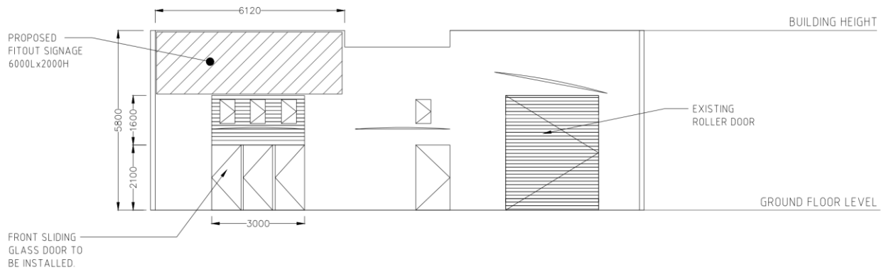
PIONEER CLOSE - ELEVATION SCALE 1:50
