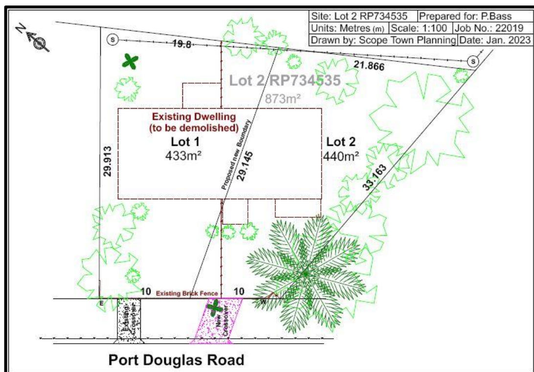
Figure 1: Proposed Site Plan (Scope Town Planning).
