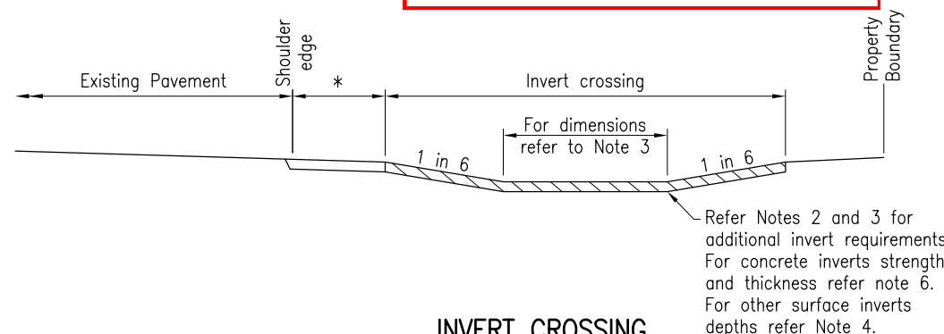
INVERT CROSSING
