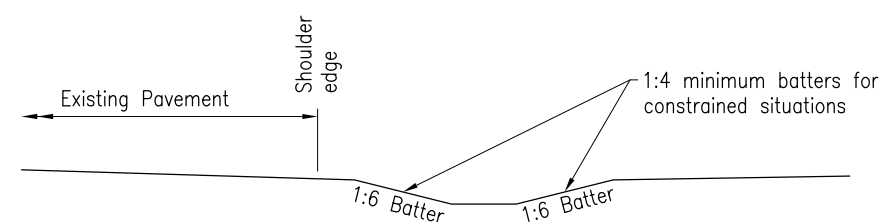
BATTER DETAIL
