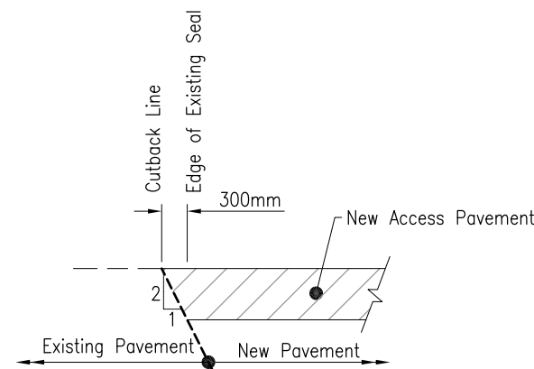
CUTBACK DETAIL
